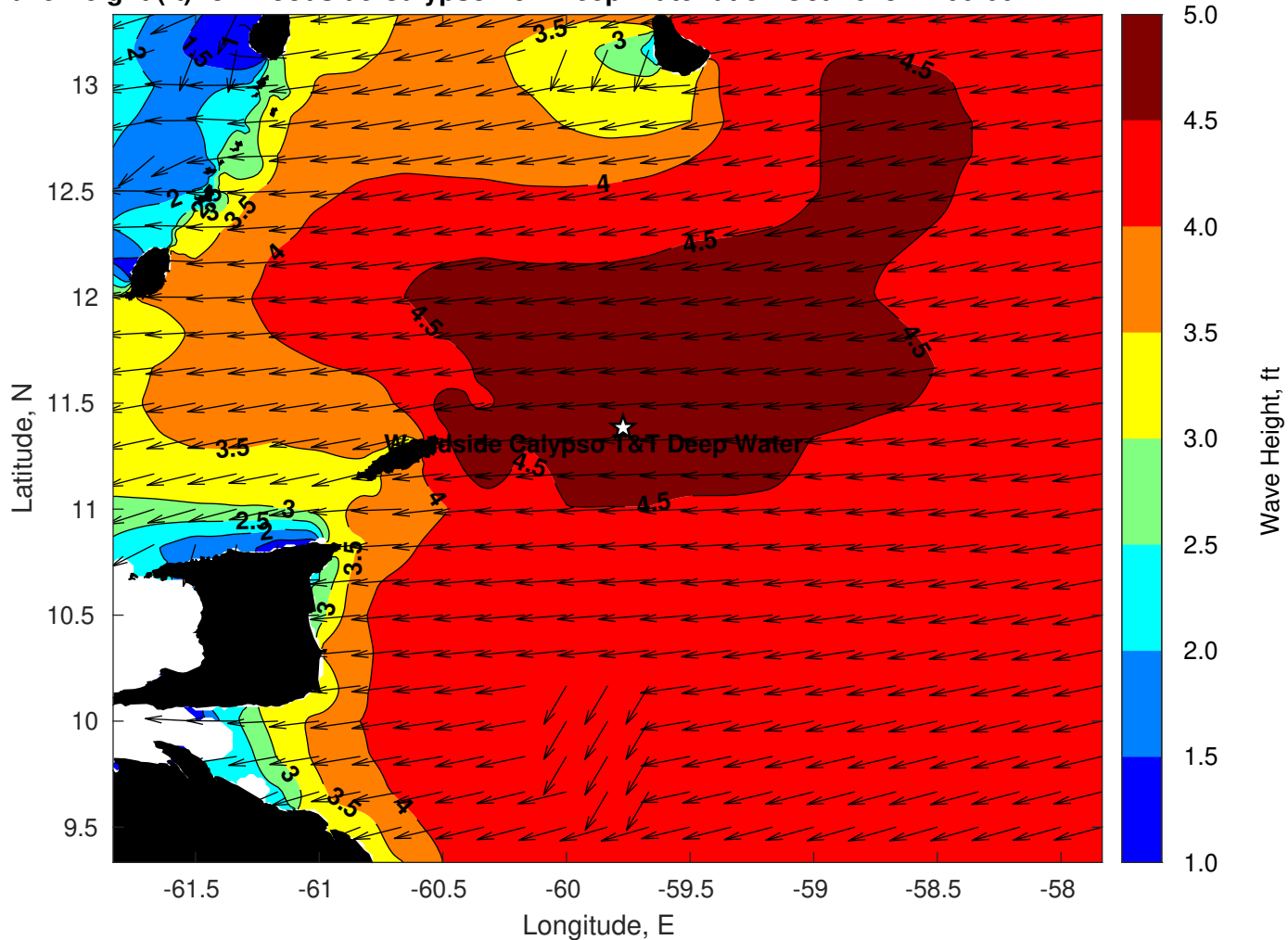
Wave Height (ft) for Woodside Calypso T&T Deep Water at 31-Oct-2023 12:00:00
