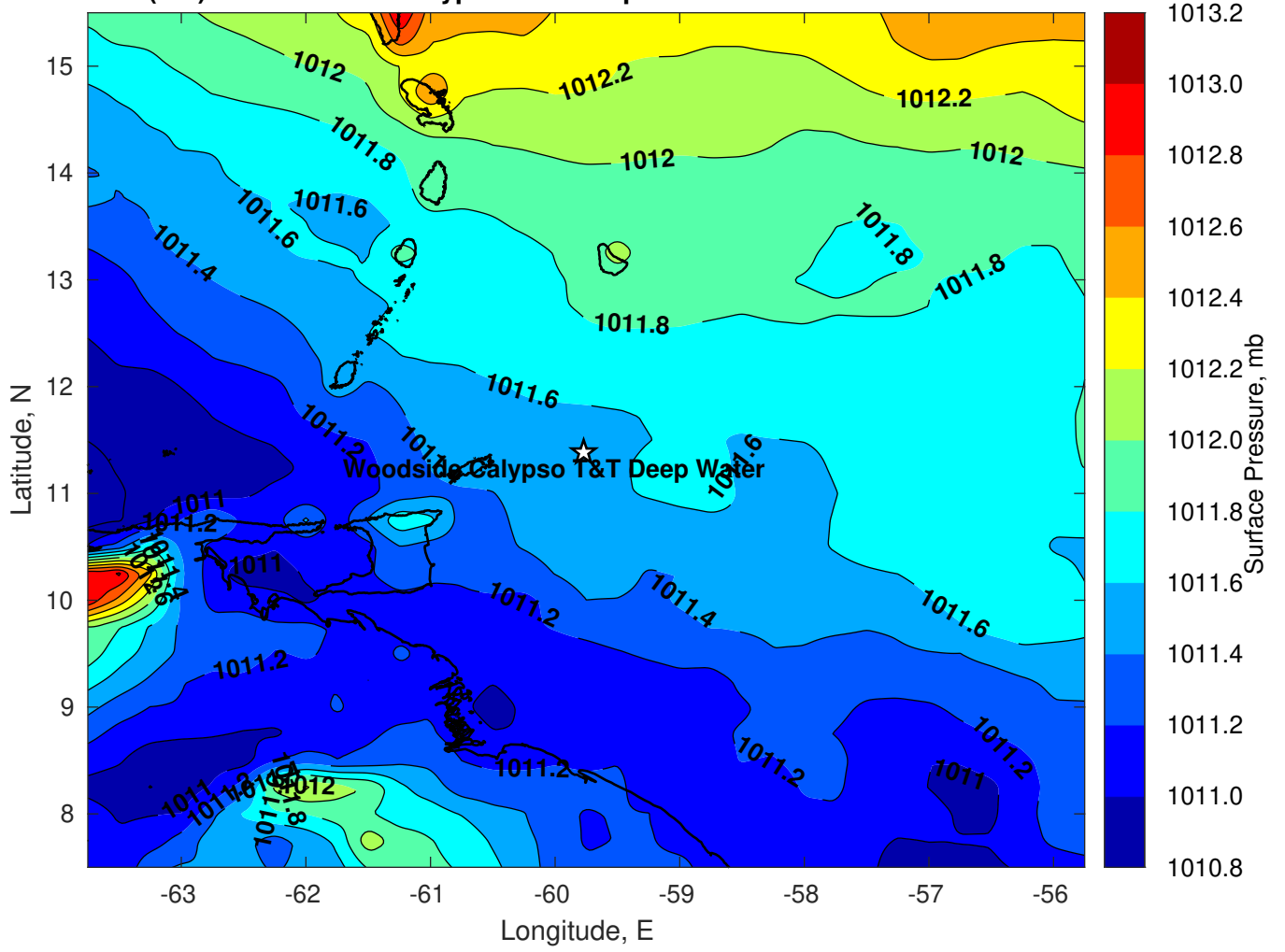
Surface Pressure (mb) for Woodside Calypso T&T Deep Water at 31-Oct-2023 12:00:00
